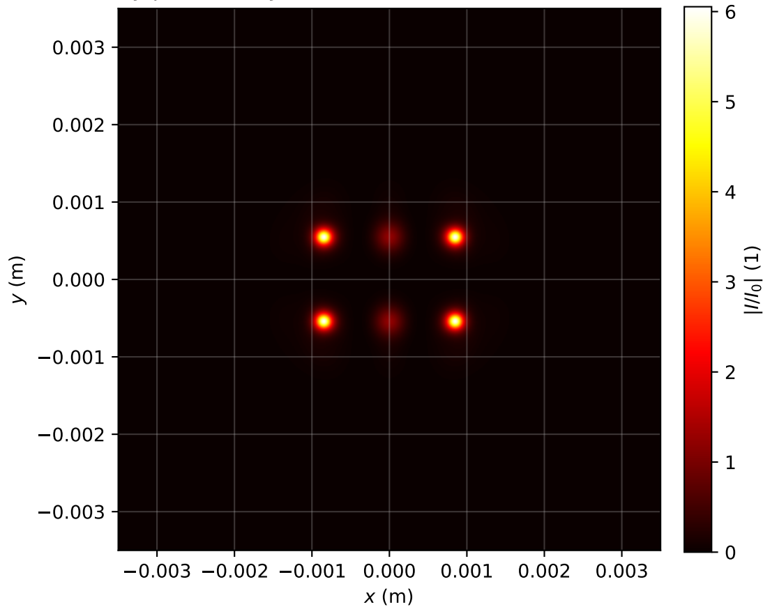
Intensity profile I(x, y, z = 0.637)/I_0 , P_{in}=6.0P_{cr} , artificial time
